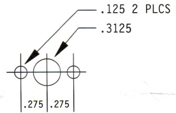
***NOT TO SCALE*** POLYCAP HOLE PATTERN
